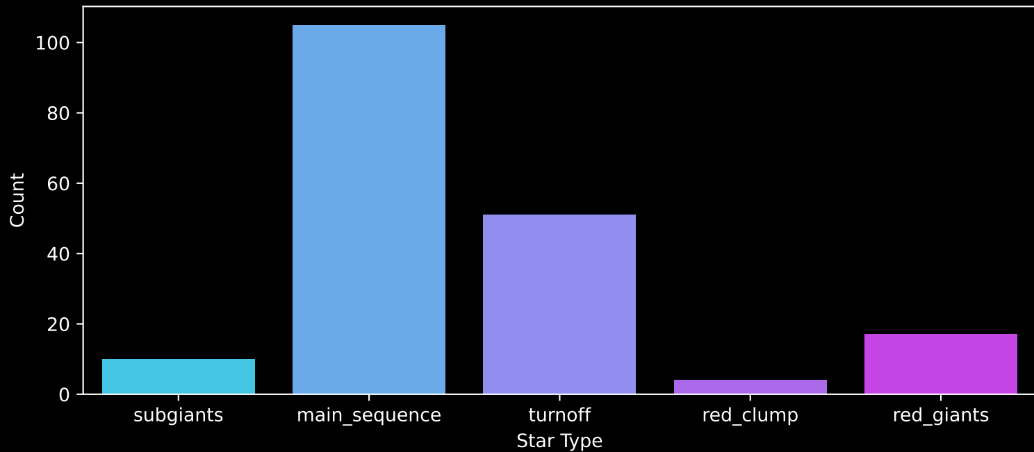
APOGEE DR17 Field: [151+79_MGA] Count plot of Star Type
