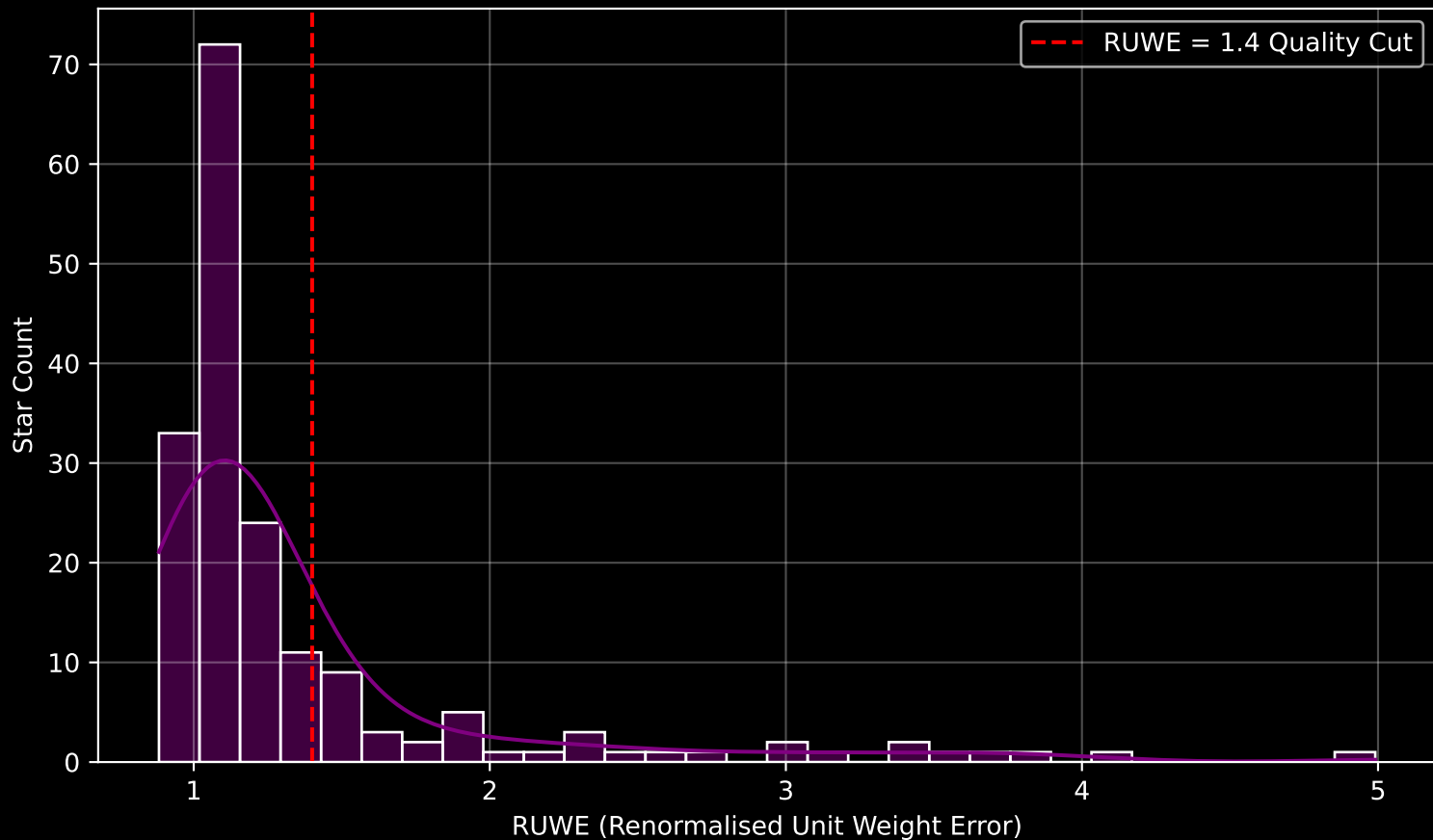
GAPOGEE DR17 Field [151+79_MGA] RUWE Distribution (n= 177)
