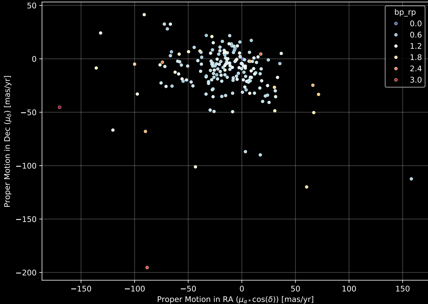
APOGEE DR17 Field: [151+79_MGA] Proper Motion Diagram (n= 187)
