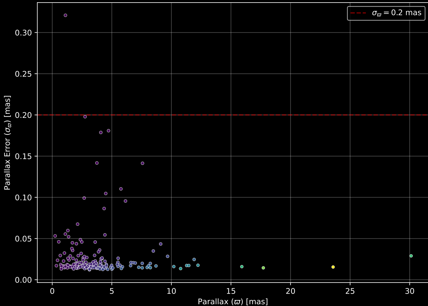
APOGEE DR17 Field: [151+79_MGA] Parallax Quality (n= 187)
