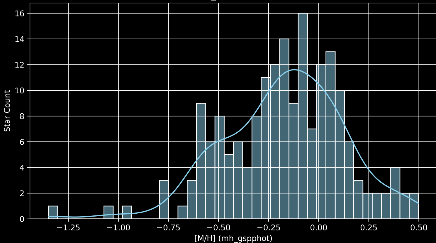
APOGEE DR17 Field: [151+79_MGA [M/H] (mh_gspphot) (n= 183)
