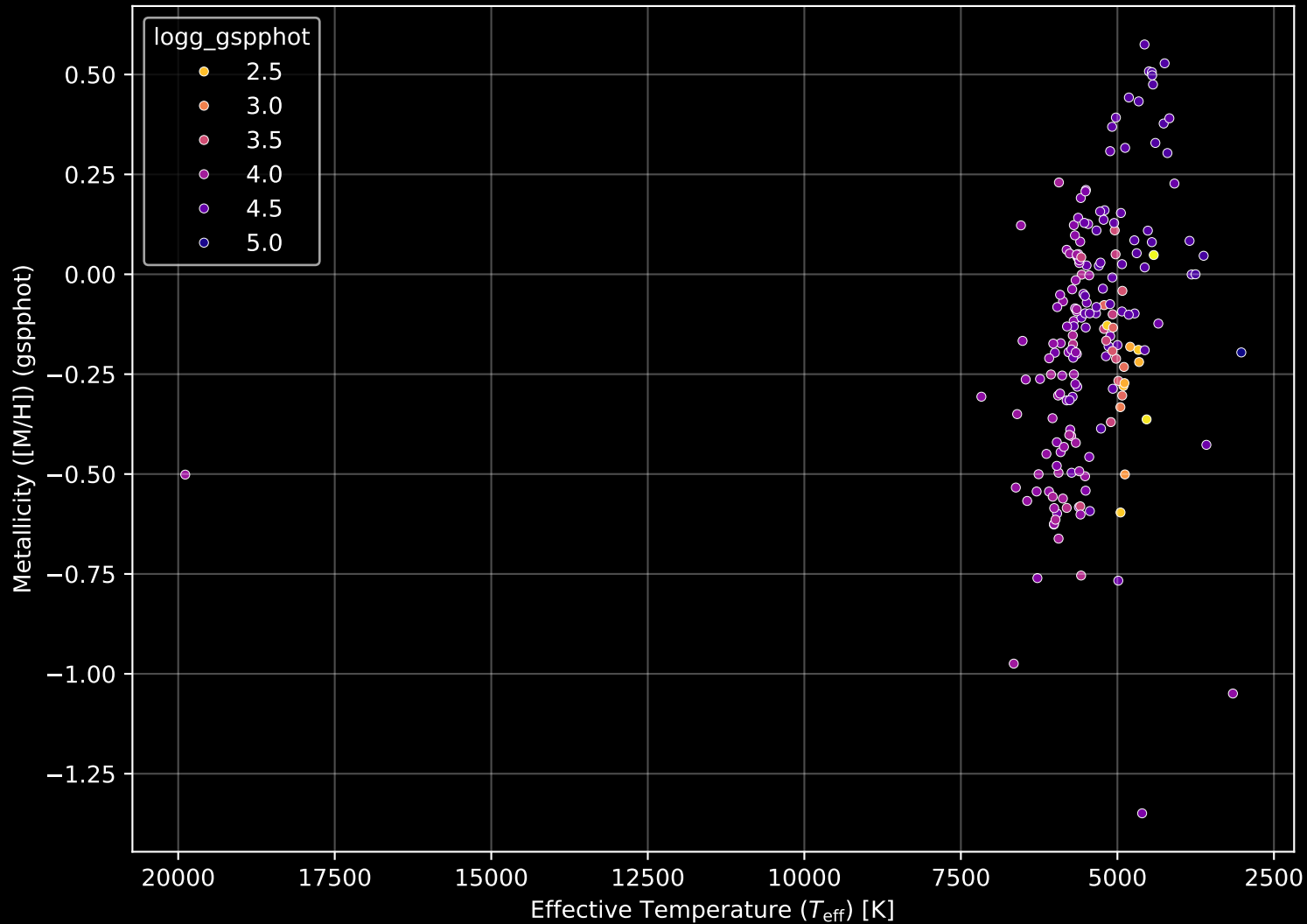
APOGEE DR17 Field: [151+79_MGA] Stellar Population Parameters (n= 187)
